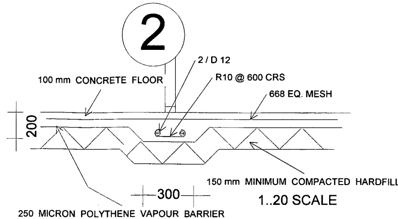
SLAB THICKENING 1..20 SCALE
