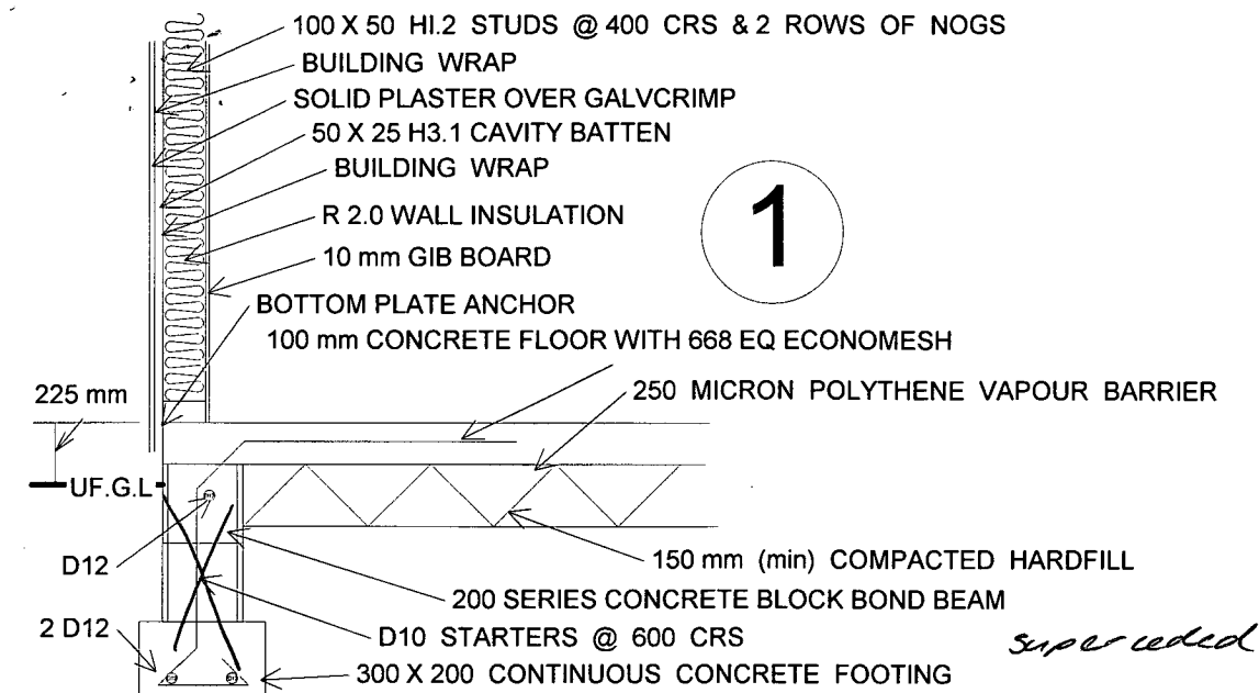
FLOOR & FOOTING DETAIL 1..20 SCALE
