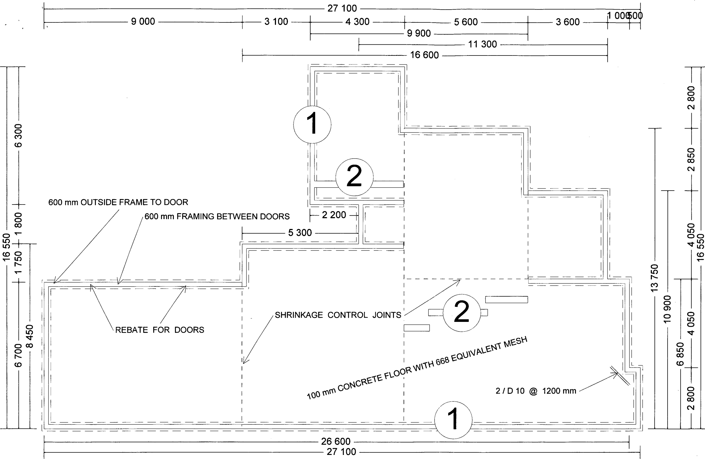
FOUNDATION PLAN 1:100 SCALE ALL DIMENSIONS ARE OUTSIDE FRAMING
