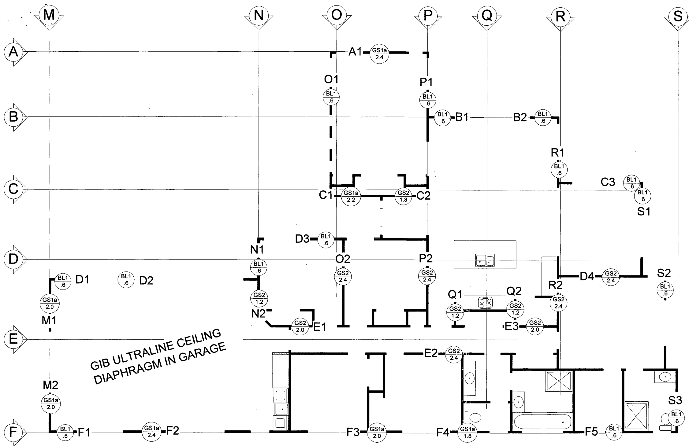
WALL BRACING PLAN 1:100 SCALE
